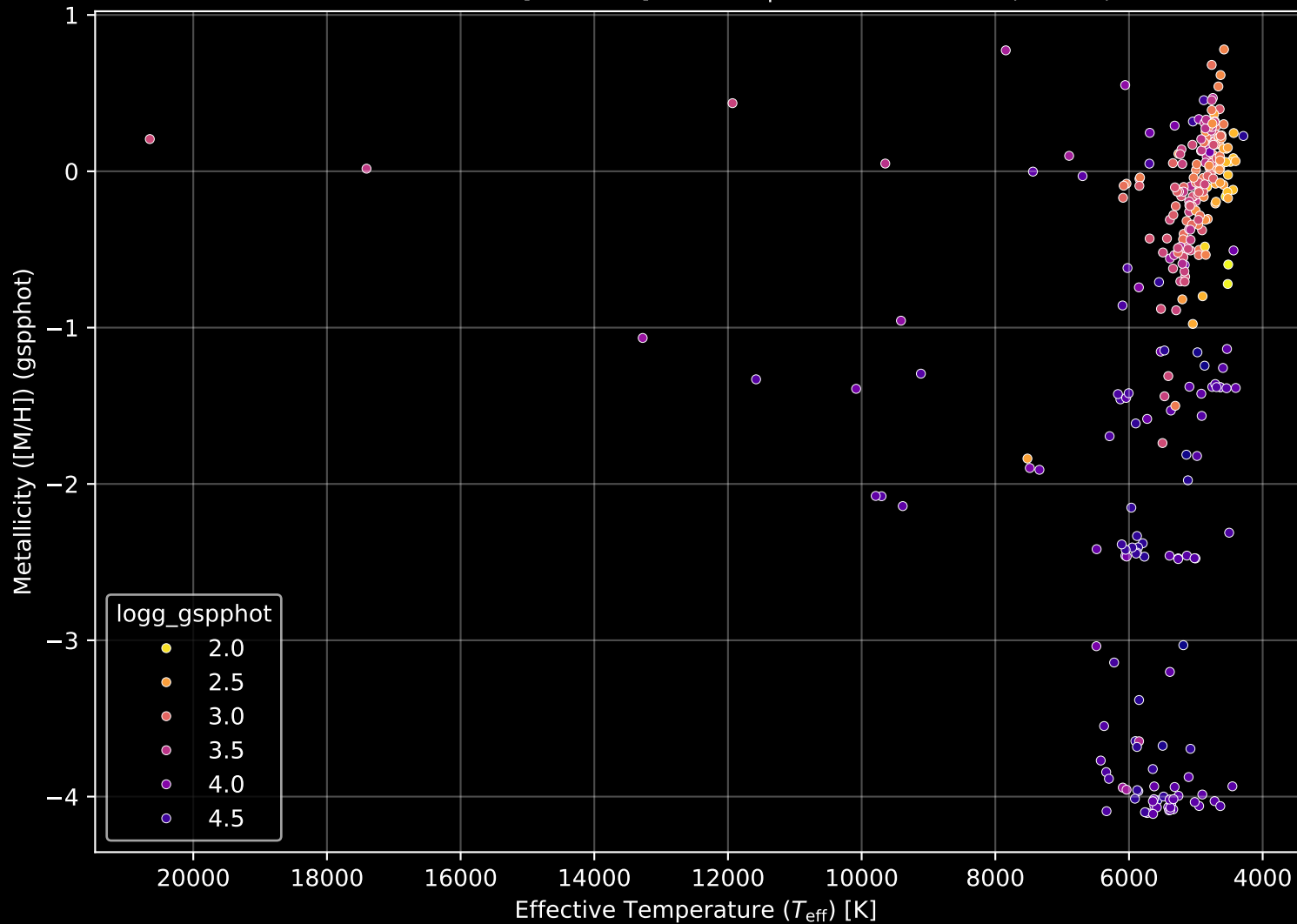
APOGEE DR17 Field: [001-04-O] Stellar Population Parameters (n= 303)
