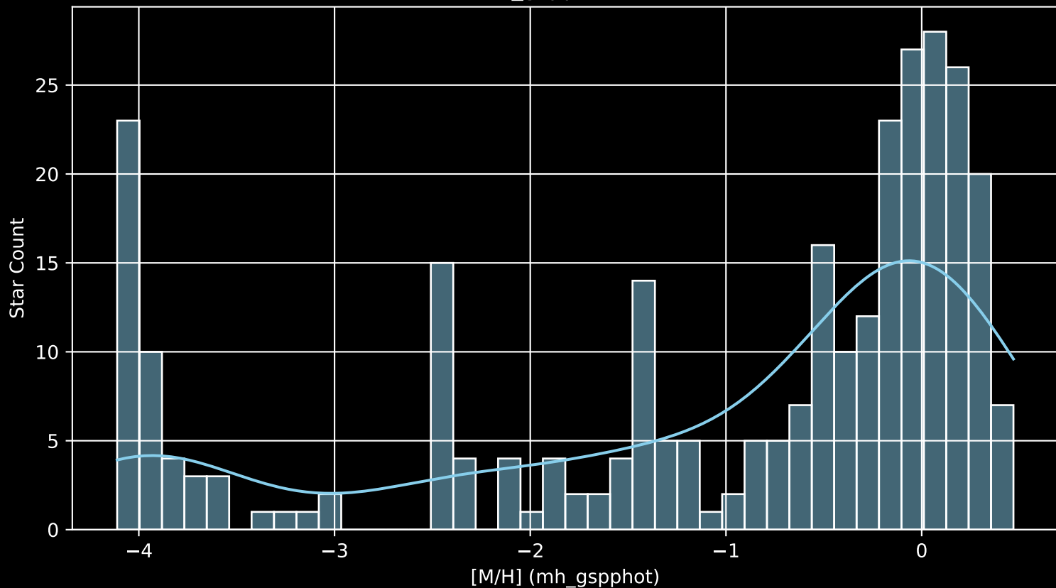
APOGEE DR17 Field: [001-04-O [M/H] (mh_gspphot) (n= 297)
