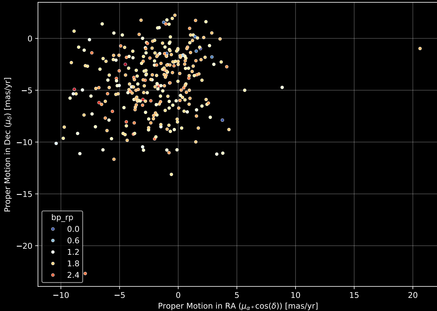
APOGEE DR17 Field: [001-04-O] Proper Motion Diagram (n= 303)
