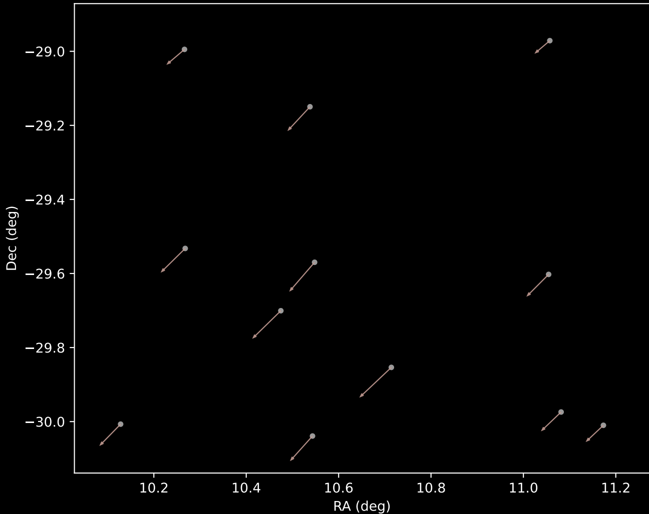
APOGEE DR17 Cluster 11 Proper Motion Vectors (n=12)
