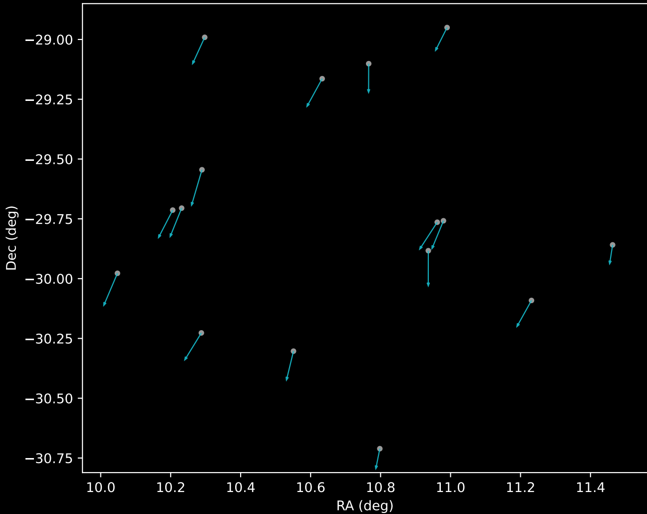
APOGEE DR17 Cluster 18 Proper Motion Vectors (n=16)
