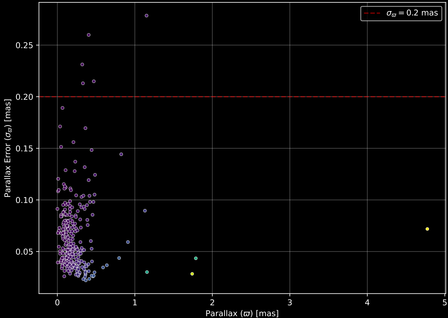
APOGEE DR17 Field: [001-04-O] Parallax Quality (n= 303)
