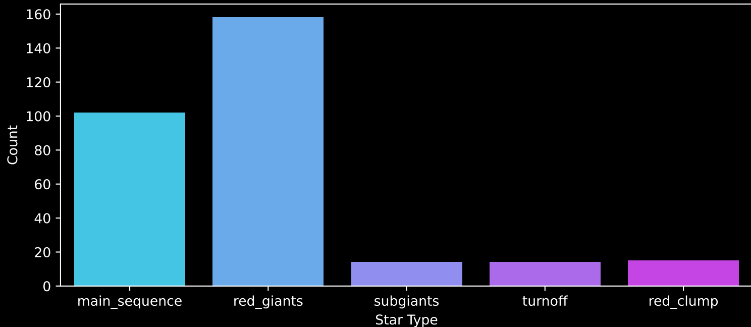
APOGEE DR17 Field: [001-04-O] Count plot of Star Type
