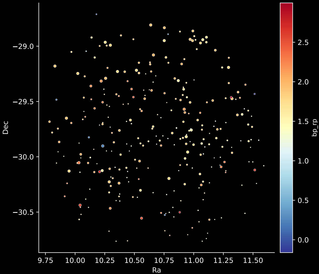
APOGEE DR17 Field: [001-04-O] Stars: 303
