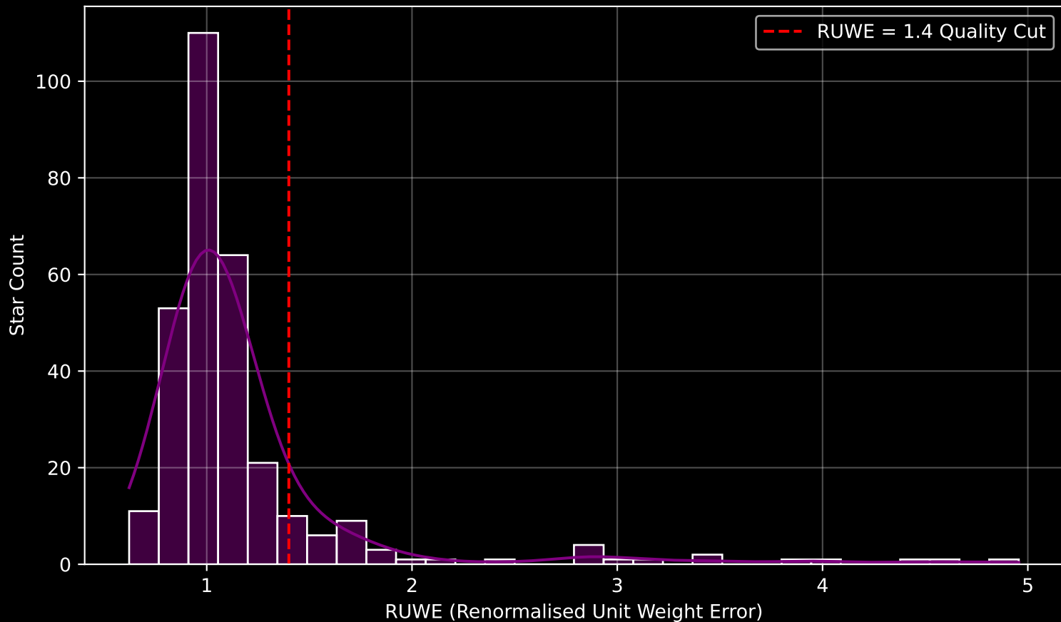
GAPOGEE DR17 Field [001-04-O] RUWE Distribution (n= 303)
